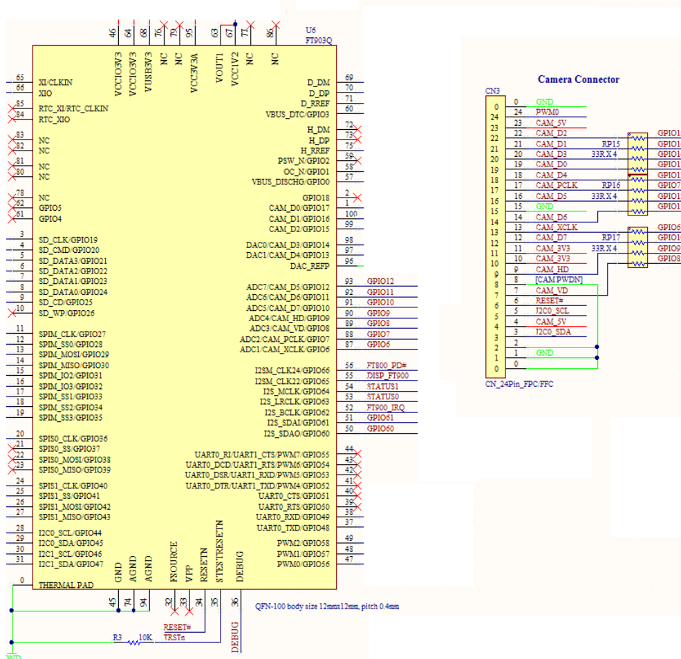
Figure 6 - Camera Interface
