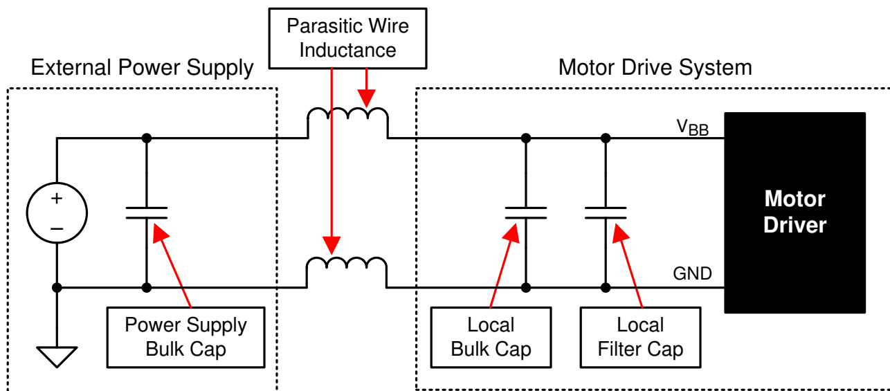
Figure 9-1. Bulk Capacitance
