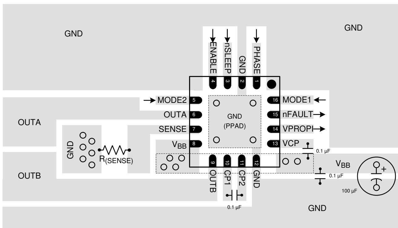
Figure 10-1. DRV8801A-Q1 Layout
