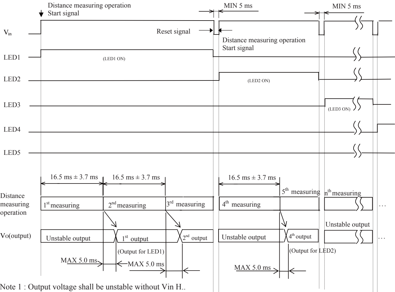
Fig. 1 Timing chart
