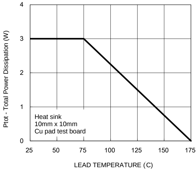
Fig.1 Steady State Power Duriating
