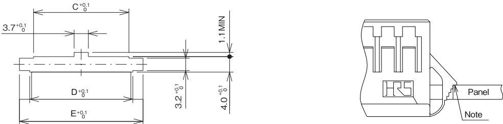
Note: Do not use a rounded surface at the panel tab portion.
