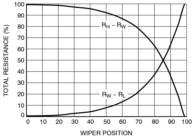
Figure 6. Wiper-Low/High Resistances vs. Wiper Position
