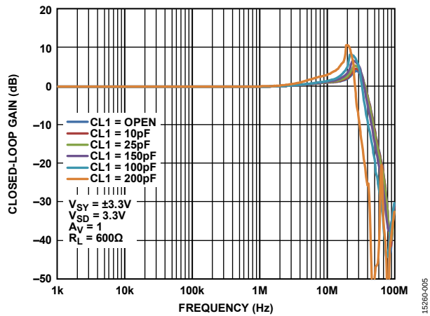
Figure 5. Frequency Response for Various Capacitive Loads, V_{SY} = \pm 3.3\text{ V}
