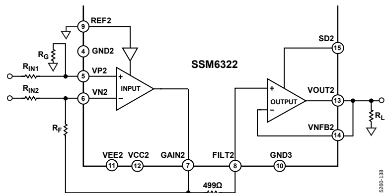
Figure 38. Test Circuit
