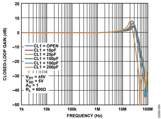
Figure 4. Frequency Response for Various Capacitive Loads, V_{SY} = \pm 5\text{ V}
