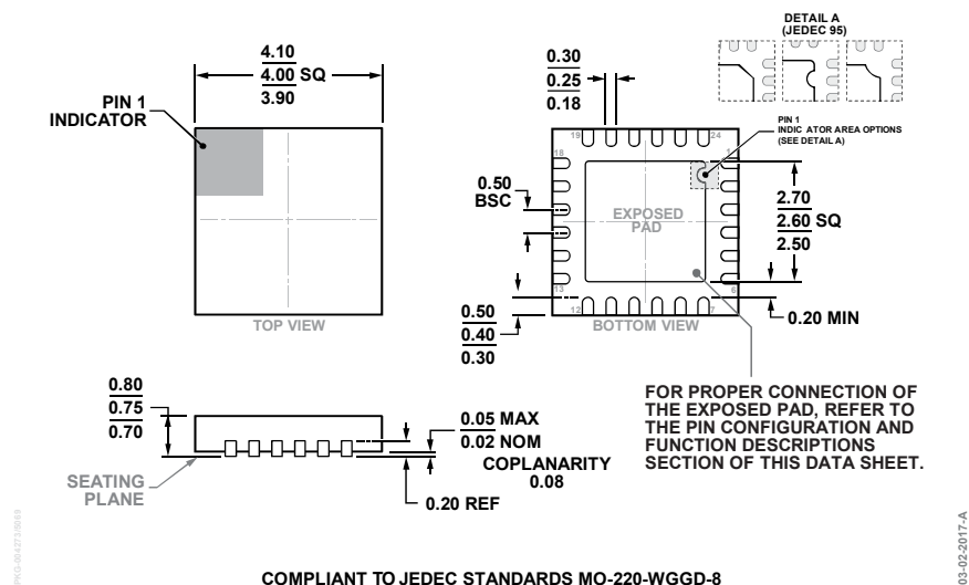
COMPLIANT TO JEDEC STANDARDS MO-220-WGGD-8 Figure 49. 24-Lead Lead Frame Chip Scale Package [LFCSP] 4 mm x 4 mm Body and 0.75 mm Package Height (CP-24-15) Dimensions shown in millimeters
