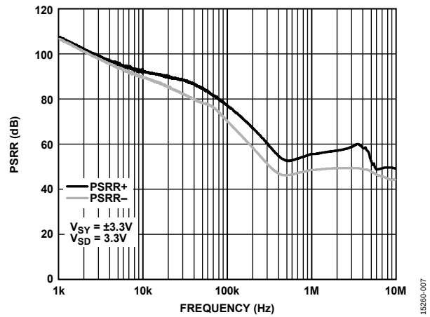
Figure 7. PSRR vs. Frequency, V_{SY} = \pm 3.3\text{ V}
