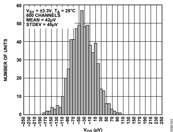
Figure 22. Input Offset Voltage ( V_{OS} ) Distribution, V_{SY} = \pm 3.3V
