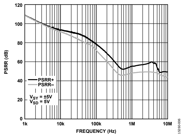
Figure 6. PSRR vs. Frequency, V_{SY} = \pm 5\text{ V}
