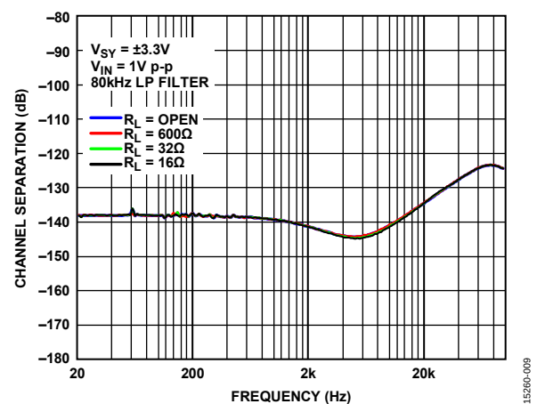
Figure 9. Channel Separation vs. Frequency, V_{SY} = \pm 3.3\text{ V}
