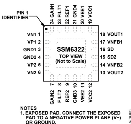
Figure 3. Pin Configuration
