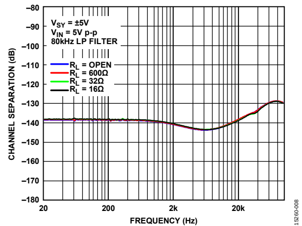
Figure 8. Channel Separation vs. Frequency, V_{SY} = \pm 5\text{ V}
