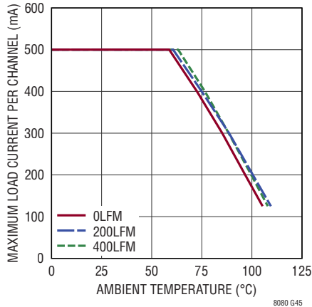
Thermal Derating 12V IN to 1.8V OUT , I BUS = I OUT1,2 = 0.5A DC3071A Demo Board
