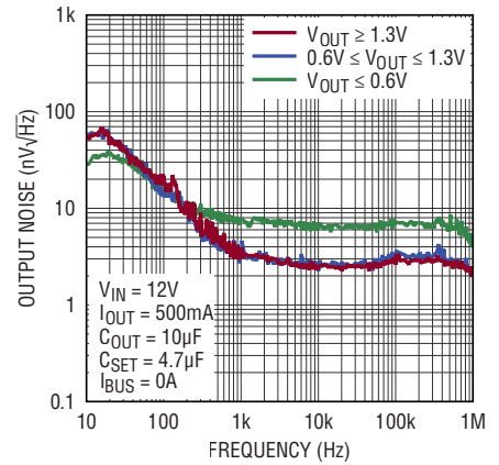
Noise Spectral Density vs V_{\text{OUT}} V_{\text{BUS}} = 2.5\text{V} or ( V_{\text{OUT1}} + 1\text{V} ), whichever is Greater
