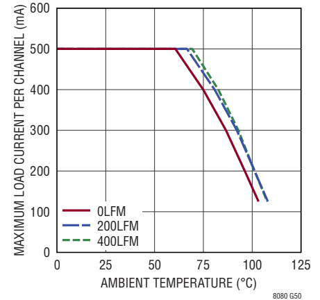
Thermal Derating 24V IN to 2.5V OUT , I BUS = I OUT1,2 = 0.5A DC3071A Demo Board
