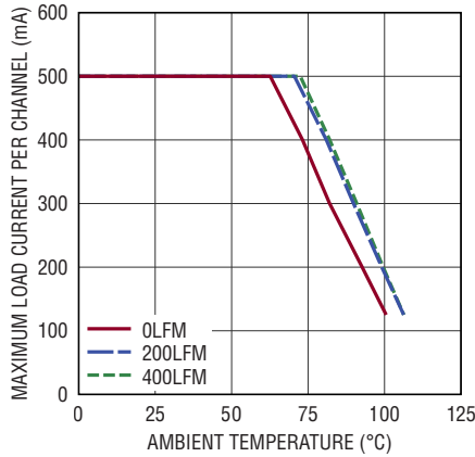
Thermal Derating 24V IN to 8V OUT , I_{\text{BUS}} = I_{\text{OUT1,2}} = 0.5\text{A} DC3071A Demo Board
