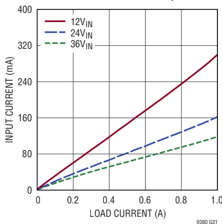
I_{IN} vs I_{OUT} , V_{OUT} = 1.8\text{V} , V_{OUT1,2} in Parallel, Burst-Mode Operation
