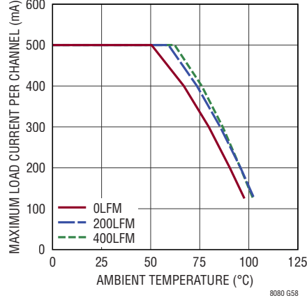
Thermal Derating 36V IN to 5V OUT , I BUS = I OUT1,2 = 0.5A DC3071A Demo Board
