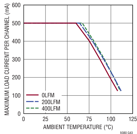
Thermal Derating 5V_{\text{IN}} to 1.2V_{\text{OUT}} , V_{\text{BUS}} = 2.5\text{V} , I_{\text{BUS}} = I_{\text{OUT1,2}} = 0.5\text{A} DC3071A Demo Board
