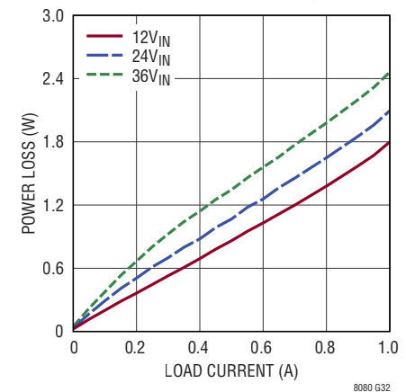
Power Loss, V_{OUT} = 1.8\text{V} , V_{OUT1,2} in Parallel, Burst-Mode Operation
