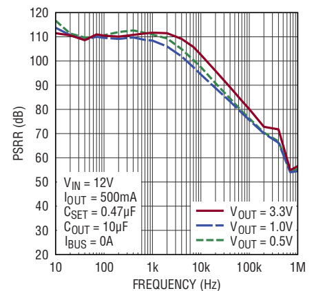
PSRR vs V_{\text{OUT}} V_{\text{BUS}} = 2.5\text{V} or ( V_{\text{OUT1}} + 1\text{V} ), whichever is Greater
