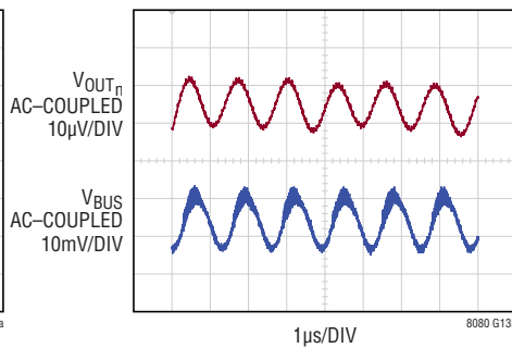
V_{\text{OUTn}} Noise Waveform V_{\text{OUTn}} : 10Hz to 1MHz BW V_{\text{BUS}} : Wideband
