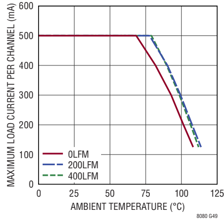
Thermal Derating 12V IN to 2.5V OUT , I BUS = I OUT1,2 = 0.5A DC3071A Demo Board
