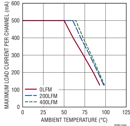
Thermal Derating 36V IN to 8V OUT , I_{\text{BUS}} = 0\text{A} , I_{\text{OUT1,2}} = 0.5\text{A} DC3071A Demo Board
