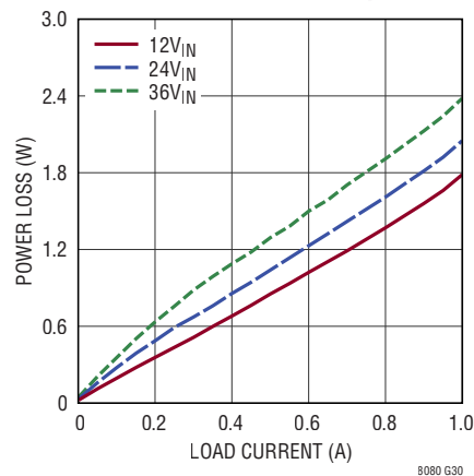
Power Loss, V_{OUT} = 1.5\text{V} , V_{OUT1,2} in Parallel, Burst-Mode Operation
