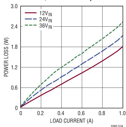
Power Loss, V_{OUT} = 2\text{V} , V_{OUT1,2} in Parallel, Burst-Mode Operation
