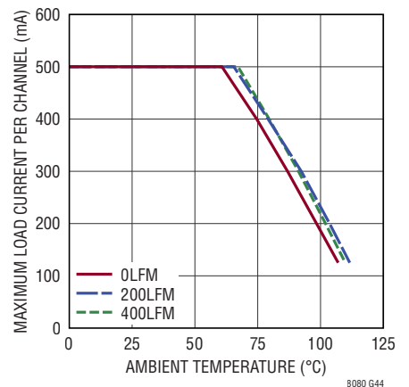
Thermal Derating 12V_{\text{IN}} to 1.2V_{\text{OUT}} , V_{\text{BUS}} = 2.5\text{V} , I_{\text{BUS}} = I_{\text{OUT1,2}} = 0.5\text{A} DC3071A Demo Board
