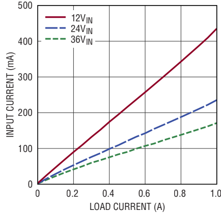
I_{\text{IN}} vs I_{\text{OUT}} , V_{\text{OUT}} = 3.3\text{V} , V_{\text{OUT1,2}} in Parallel, Burst-Mode Operation
