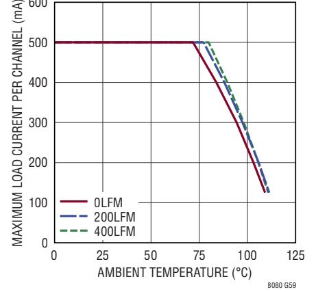
Thermal Derating 24V IN to 8V OUT , I BUS = 0A, I OUT1,2 = 0.5A DC3071A Demo Board
