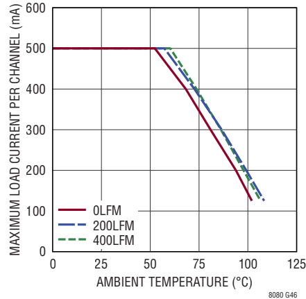
Thermal Derating 24V IN to 1.8V OUT , I BUS = I OUT1,2 = 0.5A DC3071A Demo Board
