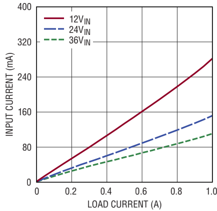
I_{IN} vs I_{OUT} , V_{OUT} = 1.2\text{V} , V_{BUS} = 2.5\text{V} , V_{OUT1,2} in Parallel, Burst-Mode Operation
