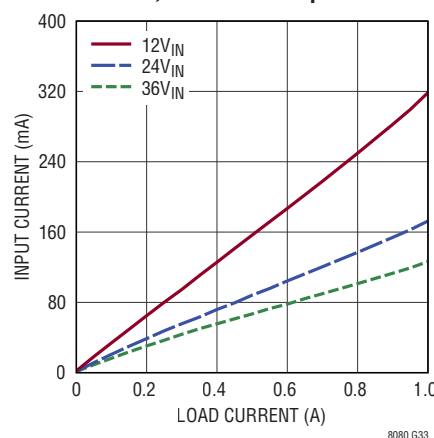
I_{IN} vs I_{OUT} , V_{OUT} = 2\text{V} , V_{OUT1,2} in Parallel, Burst-Mode Operation
