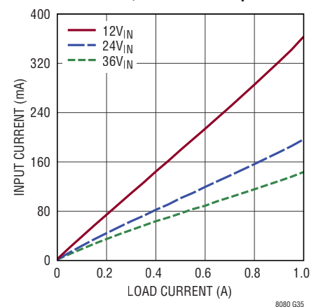
I_{IN} vs I_{OUT} , V_{OUT} = 2.5\text{V} , V_{OUT1,2} in Parallel, Burst-Mode Operation
