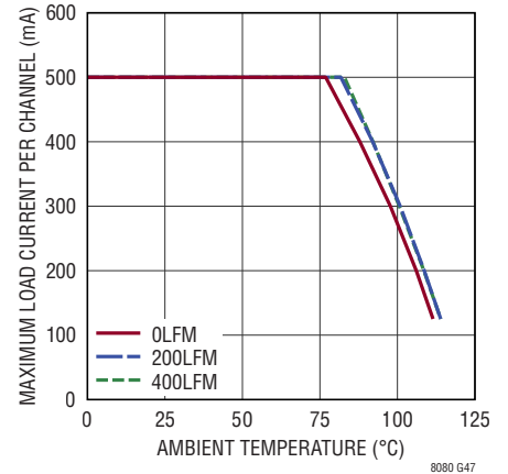
Thermal Derating 36V IN to 1.8V OUT , I BUS = I OUT1,2 = 0.5A DC3071A Demo Board
