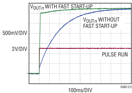
Start-Up Time with and without Fast Start-Up
