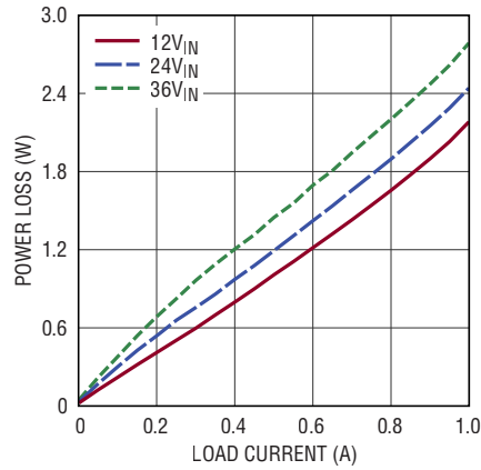
Power Loss, V_{OUT} = 1.2\text{V} , V_{BUS} = 2.5\text{V} , V_{OUT1,2} in Parallel, Burst-Mode Operation
