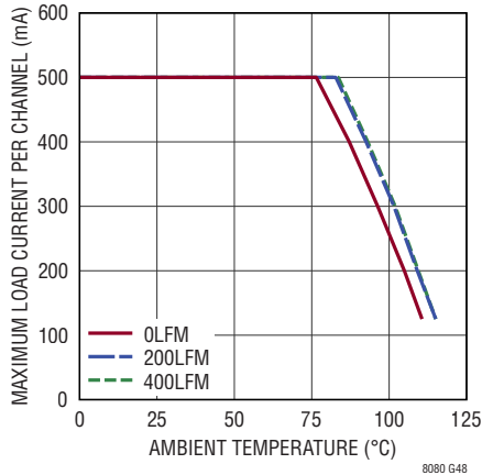
Thermal Derating 5V IN to 2.5V OUT , I BUS = I OUT1,2 = 0.5A DC3071A Demo Board
