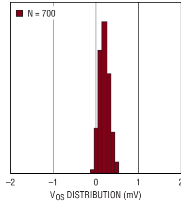
V_{\text{OS}} Distribution
