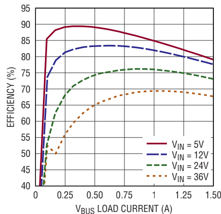
V_{\text{BUS}} Efficiency vs Load, V_{\text{BUS}} = 2.5\text{V} Pulse-Skipping Mode, f_{\text{SW}} = 800\text{kHz}
