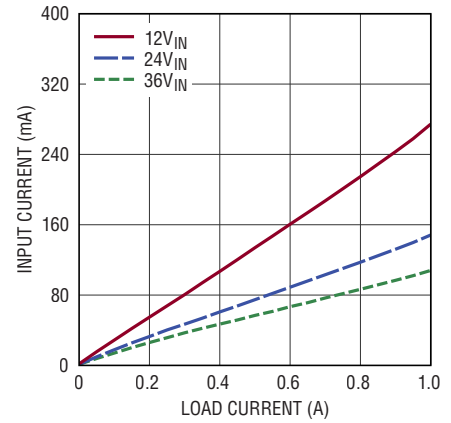
I_{IN} vs I_{OUT} , V_{OUT} = 1.5\text{V} , V_{OUT1,2} in Parallel, Burst-Mode Operation
