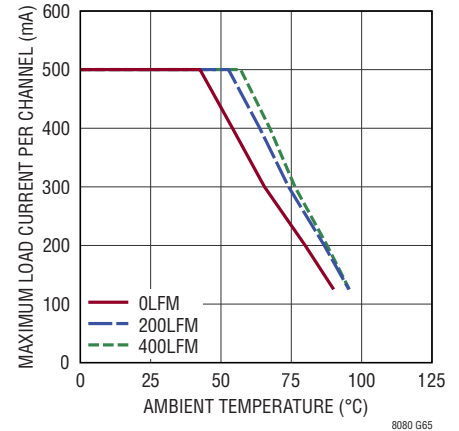
Thermal Derating 36V IN to 8V OUT , I_{\text{BUS}} = I_{\text{OUT1,2}} = 0.5\text{A} DC3071A Demo Board
