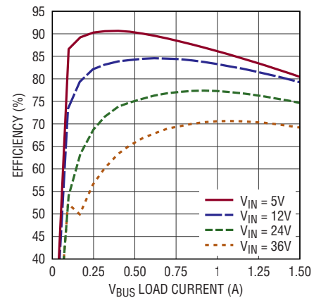
V_{\text{BUS}} Efficiency vs Load, V_{\text{BUS}} = 2.8\text{V} Pulse-Skipping Mode, f_{\text{SW}} = 900\text{kHz}
