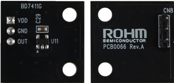
Figure 8. Board Pictures
