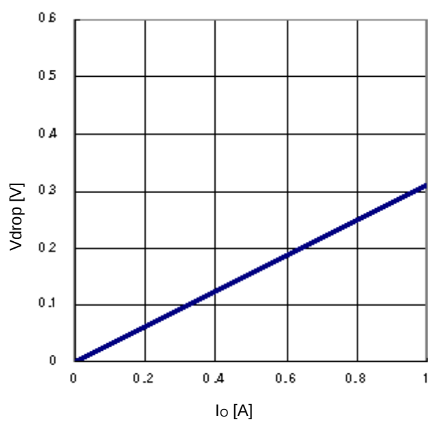
Fig.25 Minimum dropout Voltage 5 (Vcc=10V、Ta=25°C)
