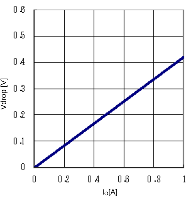
Fig.23 Minimum dropout Voltage 3 (Vcc=6V、Ta=25°C)
