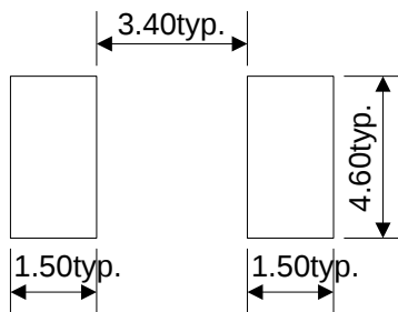
Recommended Pad Layout (mm)
