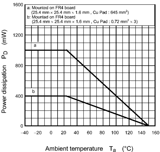
Fig. 8.14 P_D - T_a
