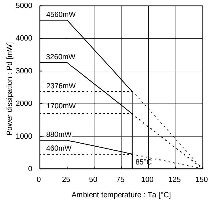
Figure 22. Package heat reduction characteristic
