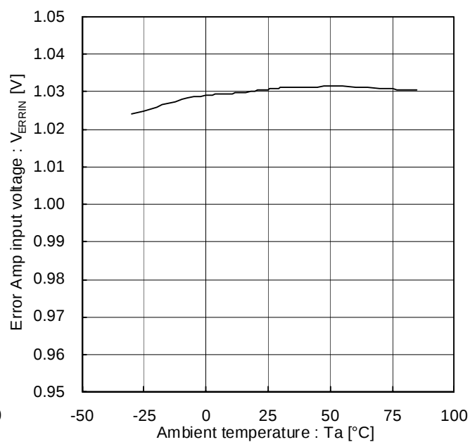
Figure 10. Error amplifier threshold voltage (Temperature dependency)
