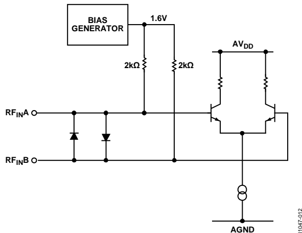
Figure 12. RF Input Stage
