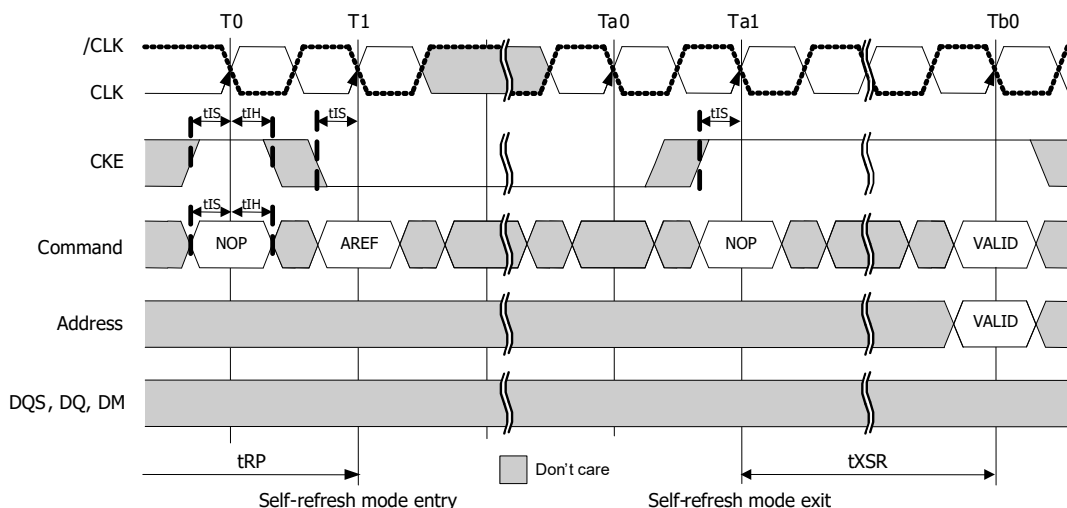
Figure 35: Self refresh
