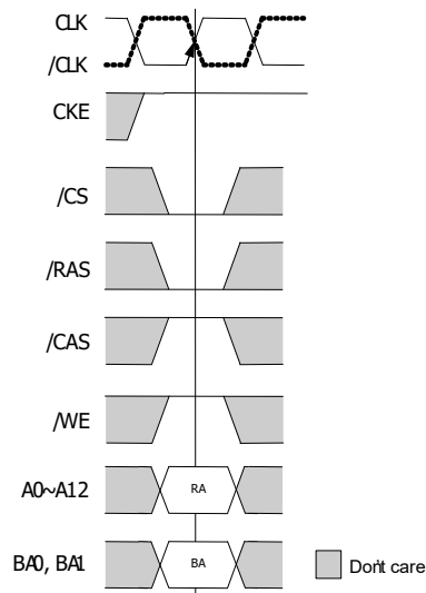
Figure 11: Active command
