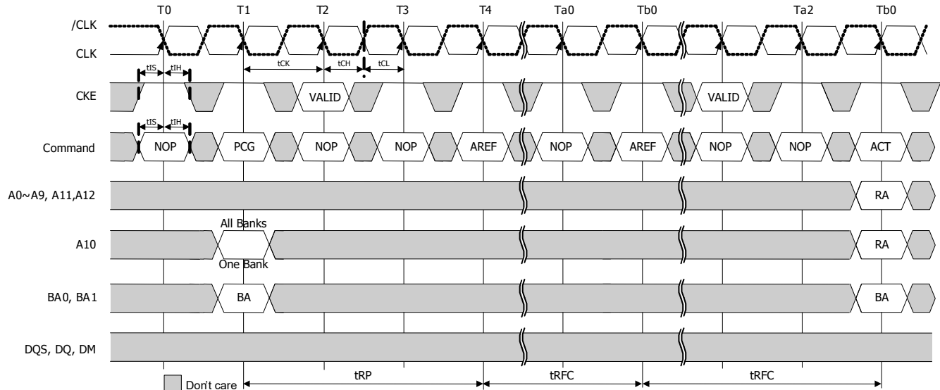
Figure 34: Auto refresh
