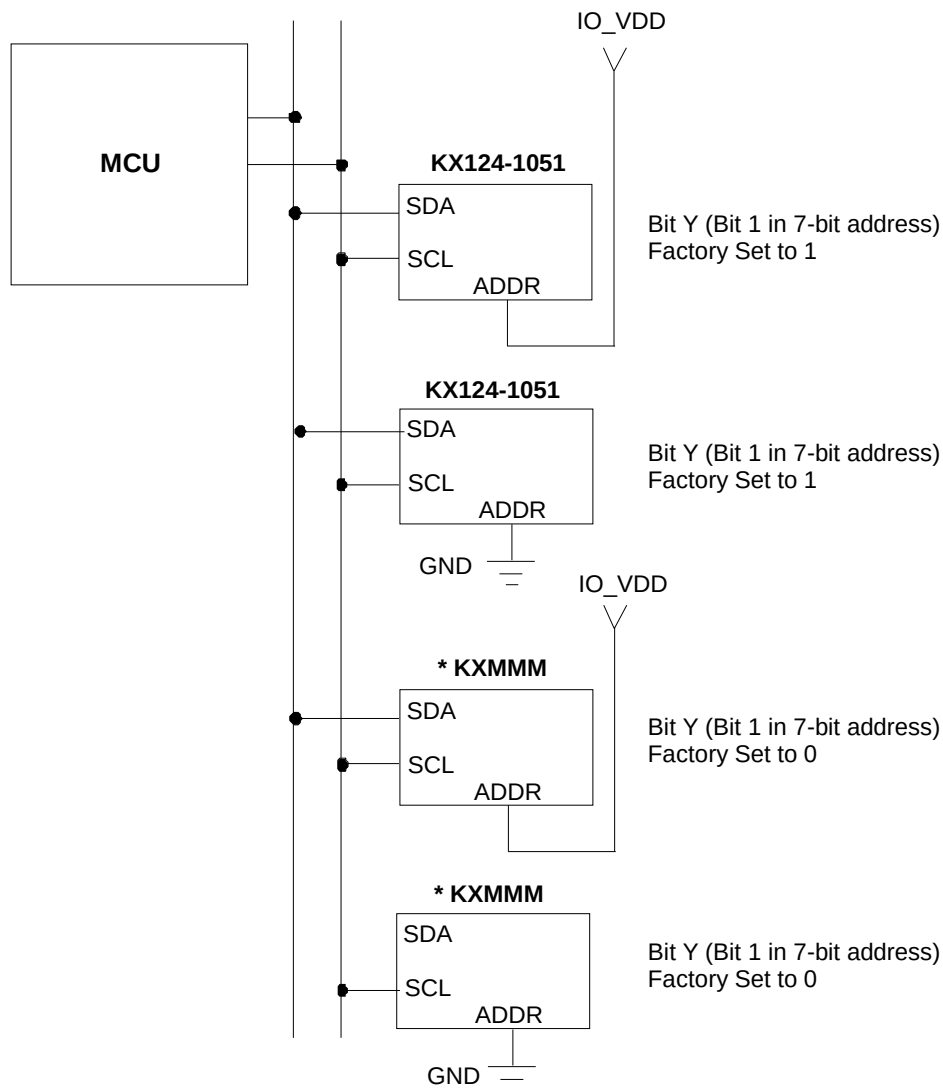
Figure 1: Multiple KX124 Accelerometers on a Shared I 2 C Bus
