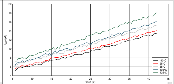
V_{CC} = 3.3\text{ V} Sleep Mode Figure 7-4. I_{SUP} vs V_{SUP} Across Temperature
