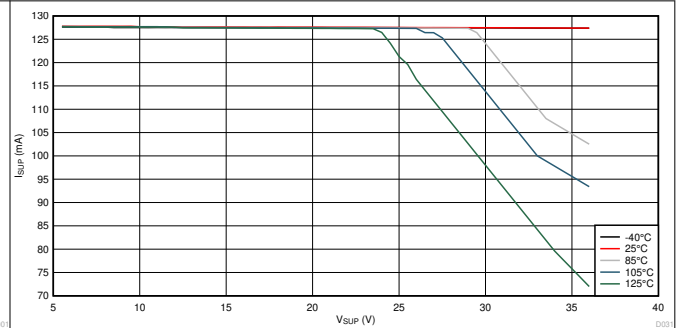
V_{CC} = 3.3\text{ V} I_{CC}\text{ Load} = 125\text{ mA} Normal Mode Figure 7-2. I_{SUP} vs V_{SUP} Across Temperature
