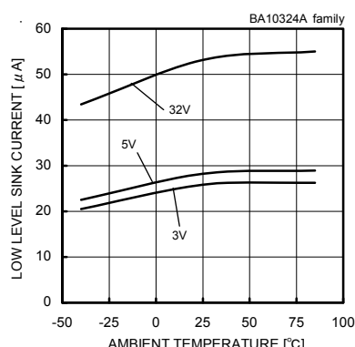
Fig. 35 Low Level Sink Current - Ambient Temperature ( V_{OUT}=0.2[V] )
