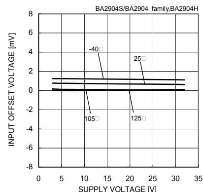
Fig. 60 Input Offset Voltage - Supply Voltage (Vcm=0[V], VOUT=1.4[V])
