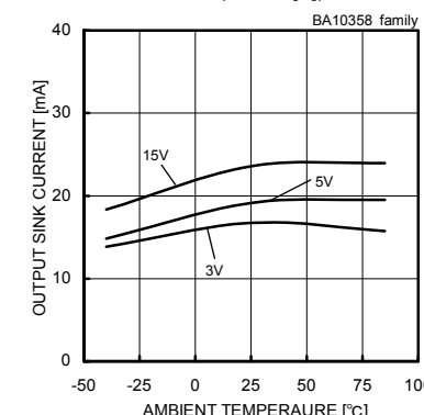
Fig. 9 Output Sink Current - Ambient Temperature ( V_{OUT}=V_{CC} )
