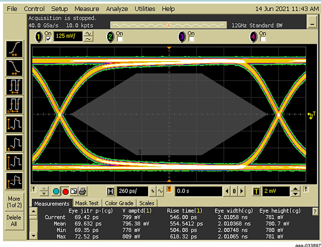
Fig. 6. USB2.0 eye diagram, Printed-Circuit Board (PCB) without device
