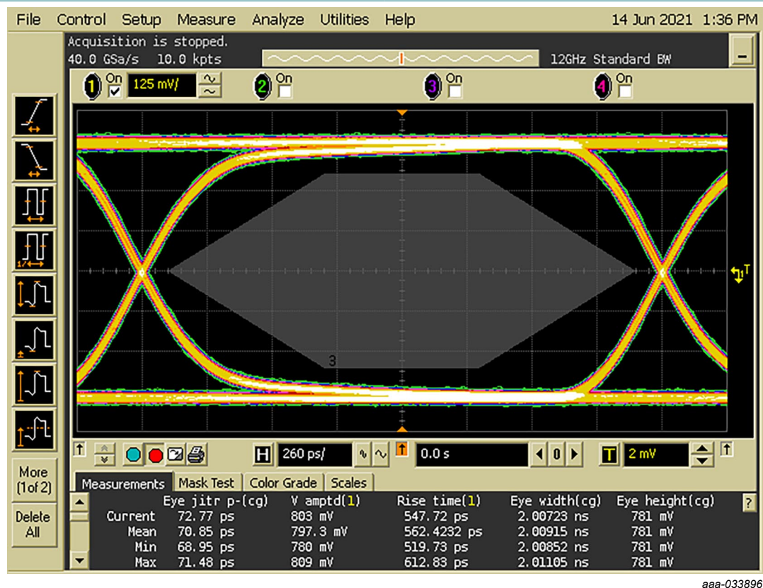
Fig. 5. USB2.0 eye diagram, Printed-Circuit Board (PCB) with device
