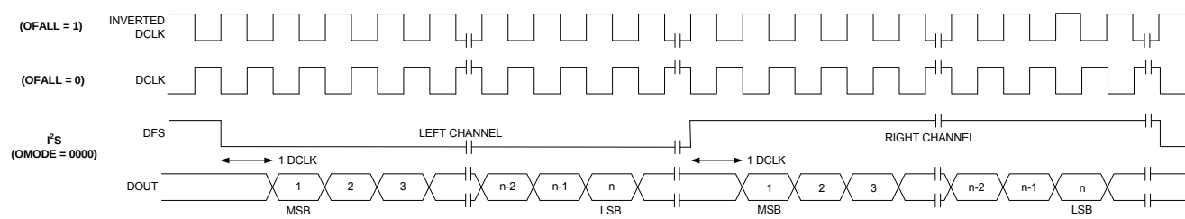
Figure 8. I²S Digital Audio Format
