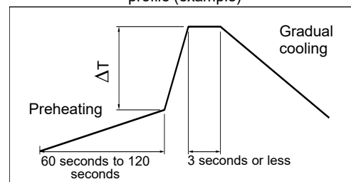
Recommended soldering-iron-used soldering profile (example)
