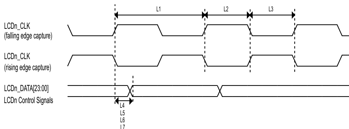
Figure 14. LCD timing
