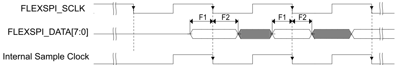
Figure 44. FlexSPI input timing in SDR mode where FlexSPI IN _MCR0[RXCLKSRC] = 0X0, 0X1
