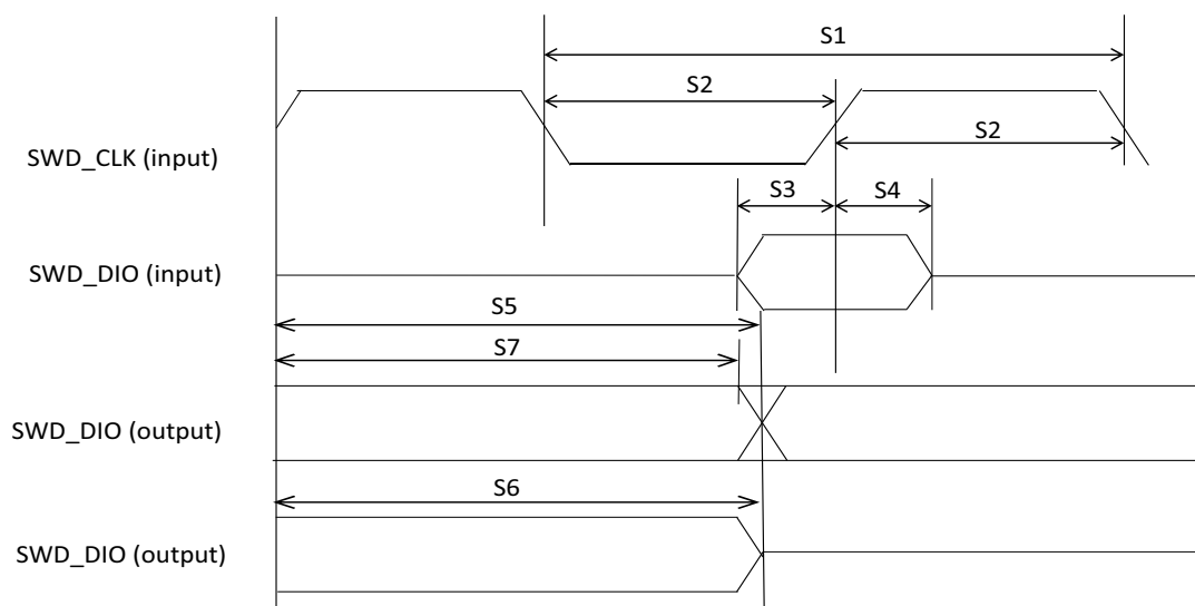
Figure 13. SWD timing
