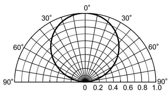
Fig. 8.7 Radiation Pattern
