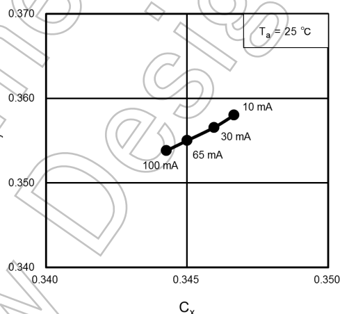
Fig. 8.4 Chromaticity - I_F
