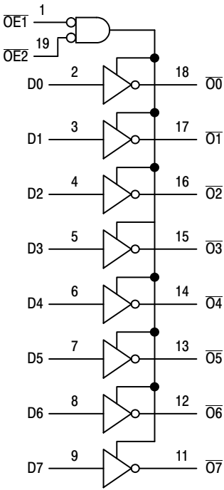
Figure 2. Logic Diagram
