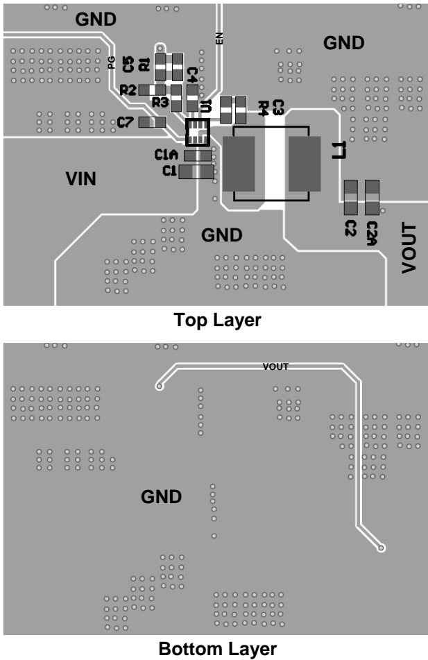
Figure 5: Recommended Layout
