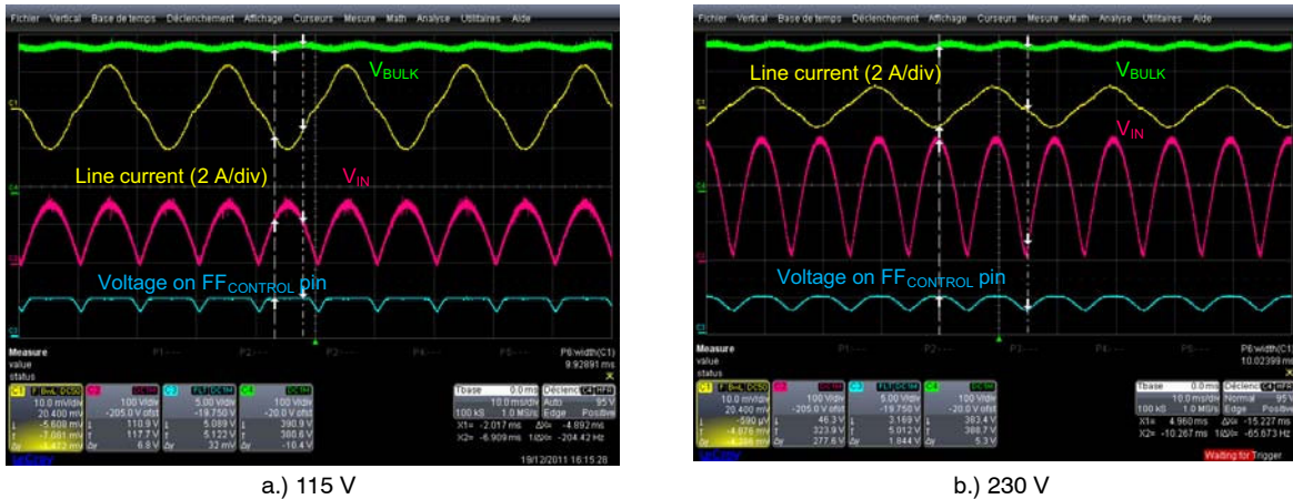
Figure 4. General Waveforms at Full Load
