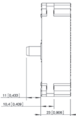
Rack guide
