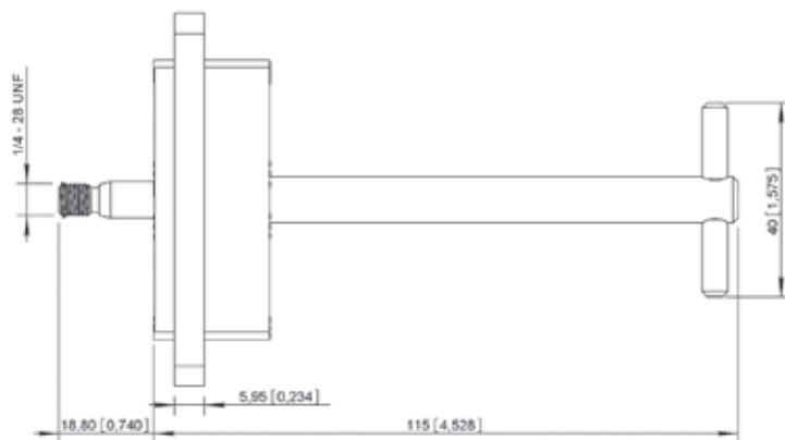
Central jackscrew
