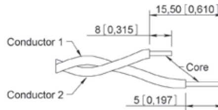
PIN CONTACT
