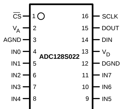
Figure 1. TSSOP
