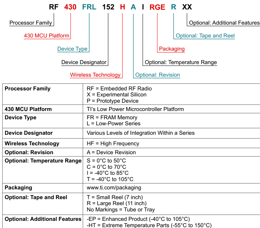
Figure 8-1. Device Nomenclature
