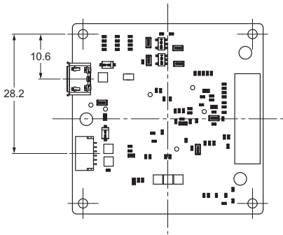
Main Board Front
