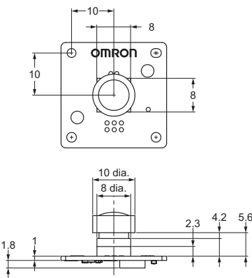
Horizontal angle of view 90° B5T-007001-020
