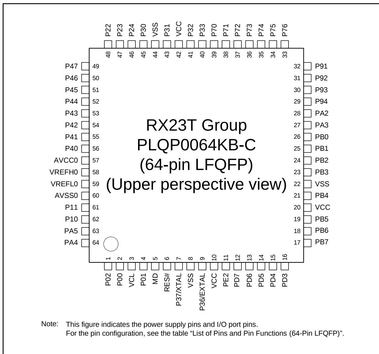
Figure 1.3 Pin Assignments of the 64-Pin LFQFP
