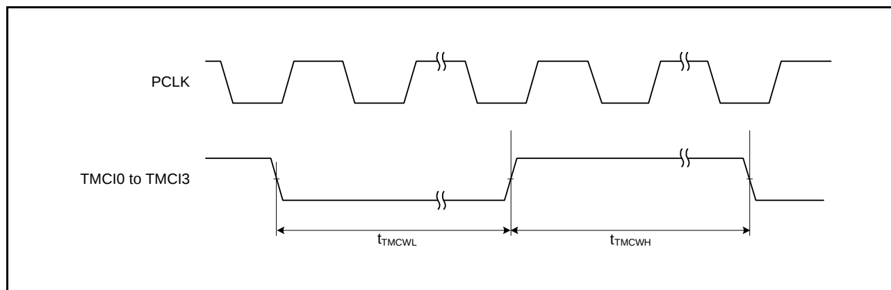
Figure 5.38 TMR Clock Input Timing
