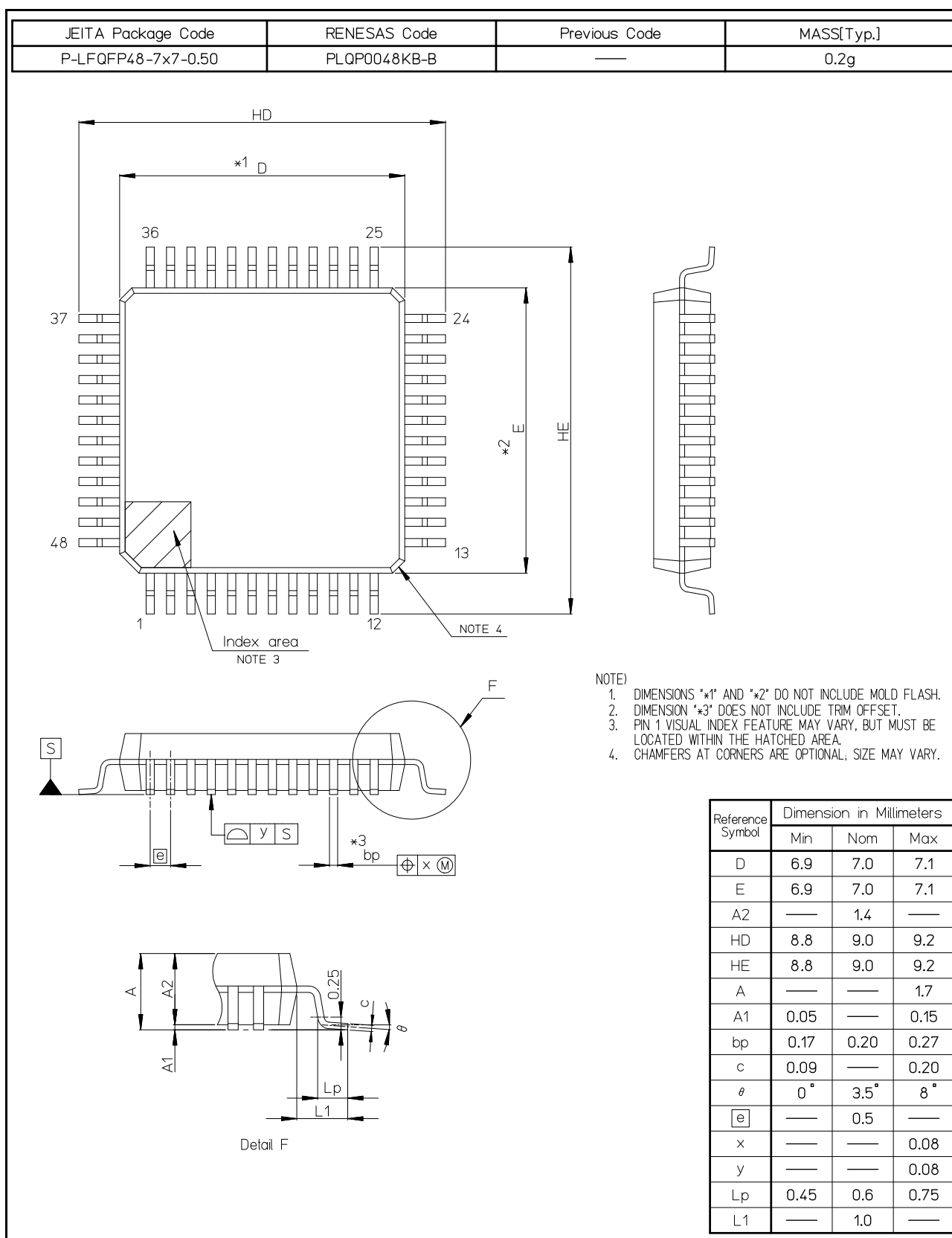
Figure C 48-Pin LFQFP (PLQP0048KB-B)
