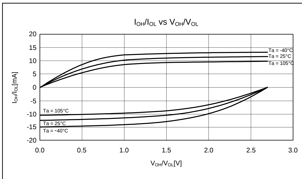
Figure 5.5 V_{OH}/V_{OL} and I_{OH}/I_{OL} Temperature Characteristics at V_{CC} = 2.7 \text{ V} when Normal Output is Selected (Reference Data)
