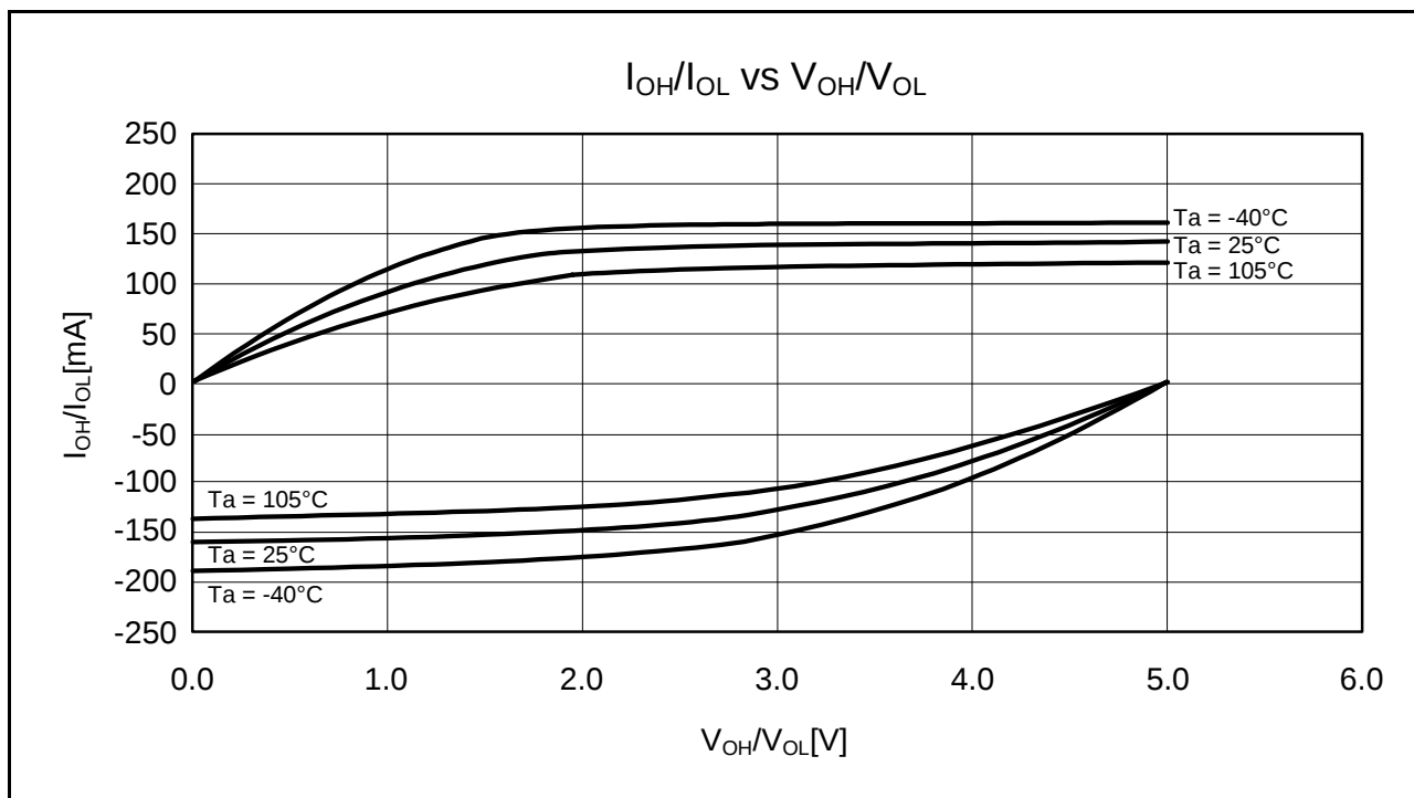
Figure 5.14 V_{OH}/V_{OL} and I_{OH}/I_{OL} Temperature Characteristics of Large Current Ports (Ports 71 to 76, Port B5, Port D3) at V_{CC} = 5.0 V (Reference Data)
