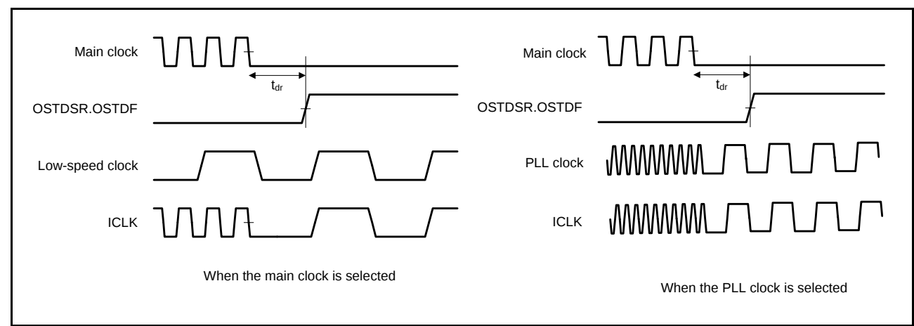
Figure 5.55 Oscillation Stop Detection Timing
