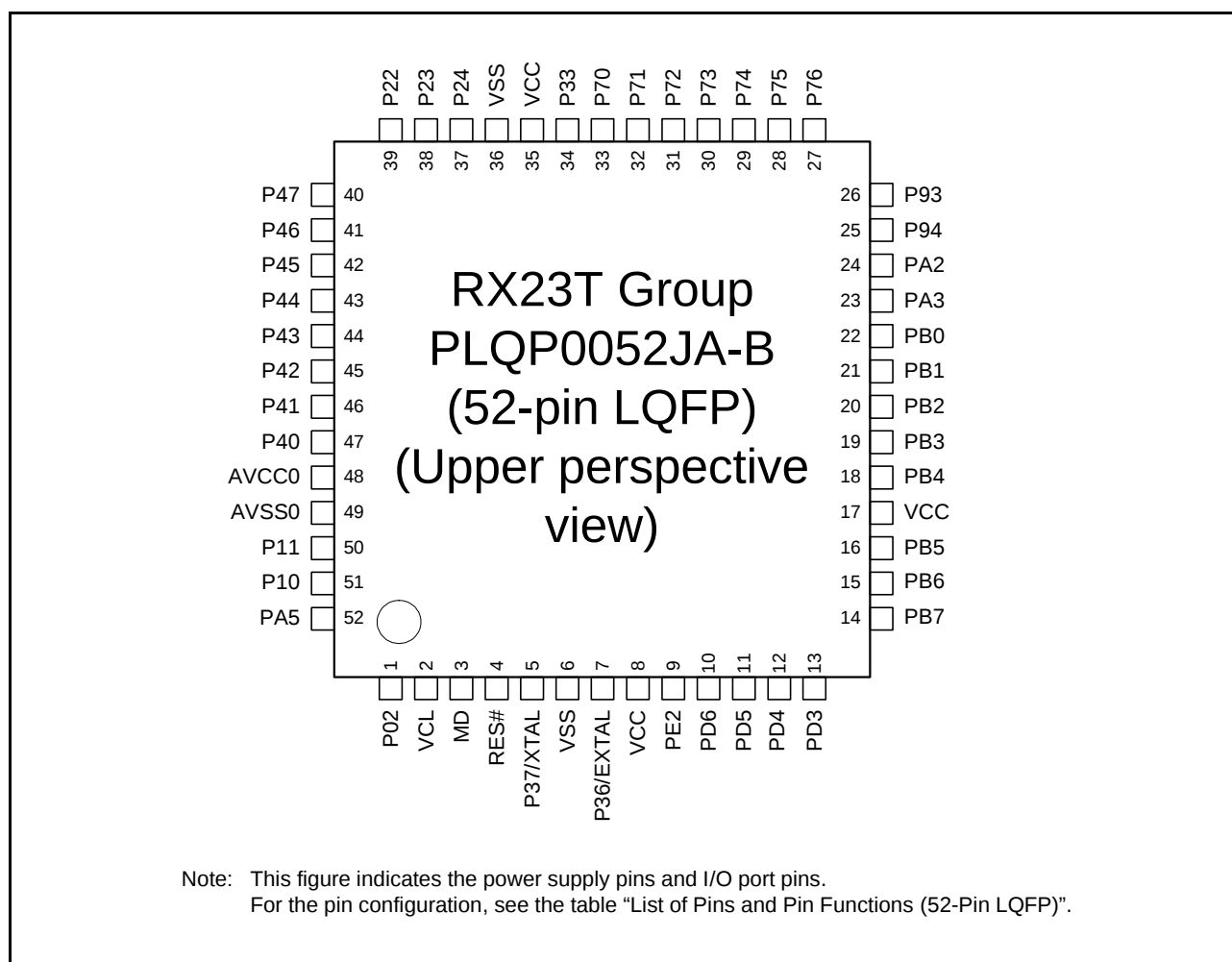
Figure 1.4 Pin Assignments of the 52-Pin LQFP
