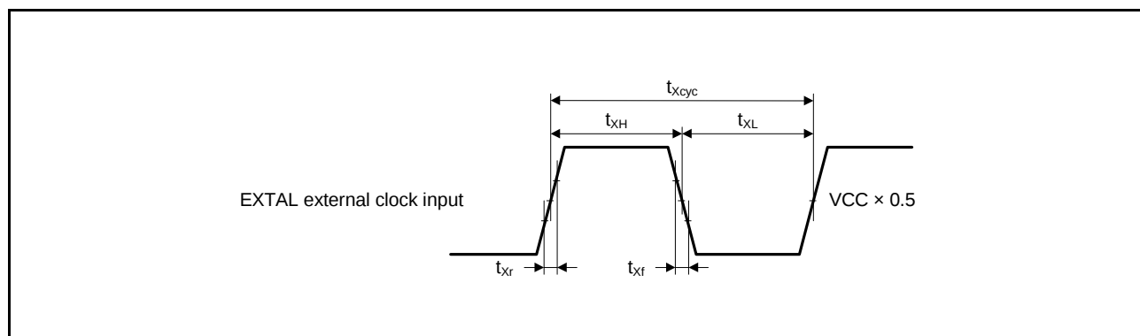
Figure 5.20 EXTAL External Clock Input Timing
