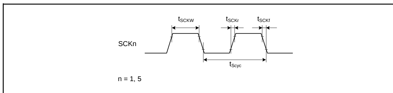
Figure 5.39 SCK Clock Input Timing
