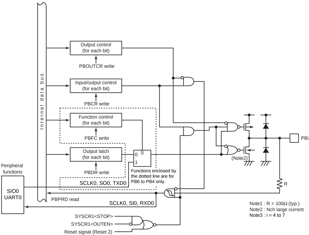
Figure 8-10 Port PB
