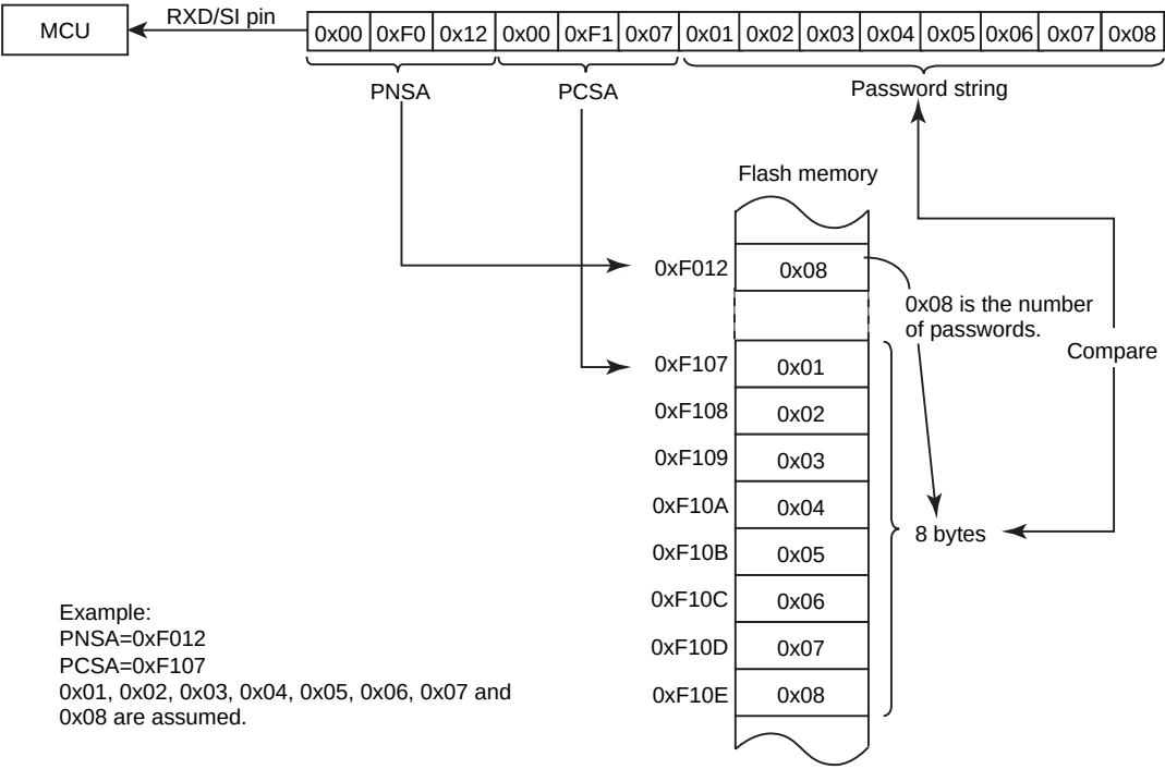
Figure 22-4 Password Structure (Example of a Password Transmitted)
