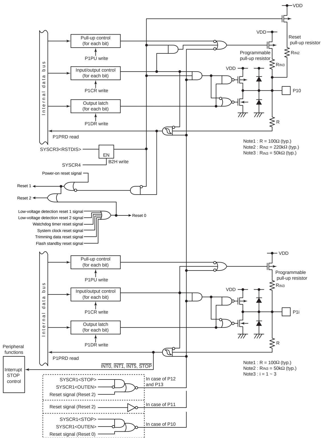
Figure 8-4 Port P1
