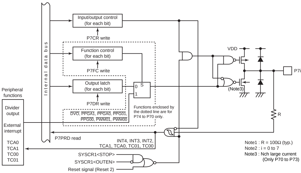
Figure 8-7 Port P7
