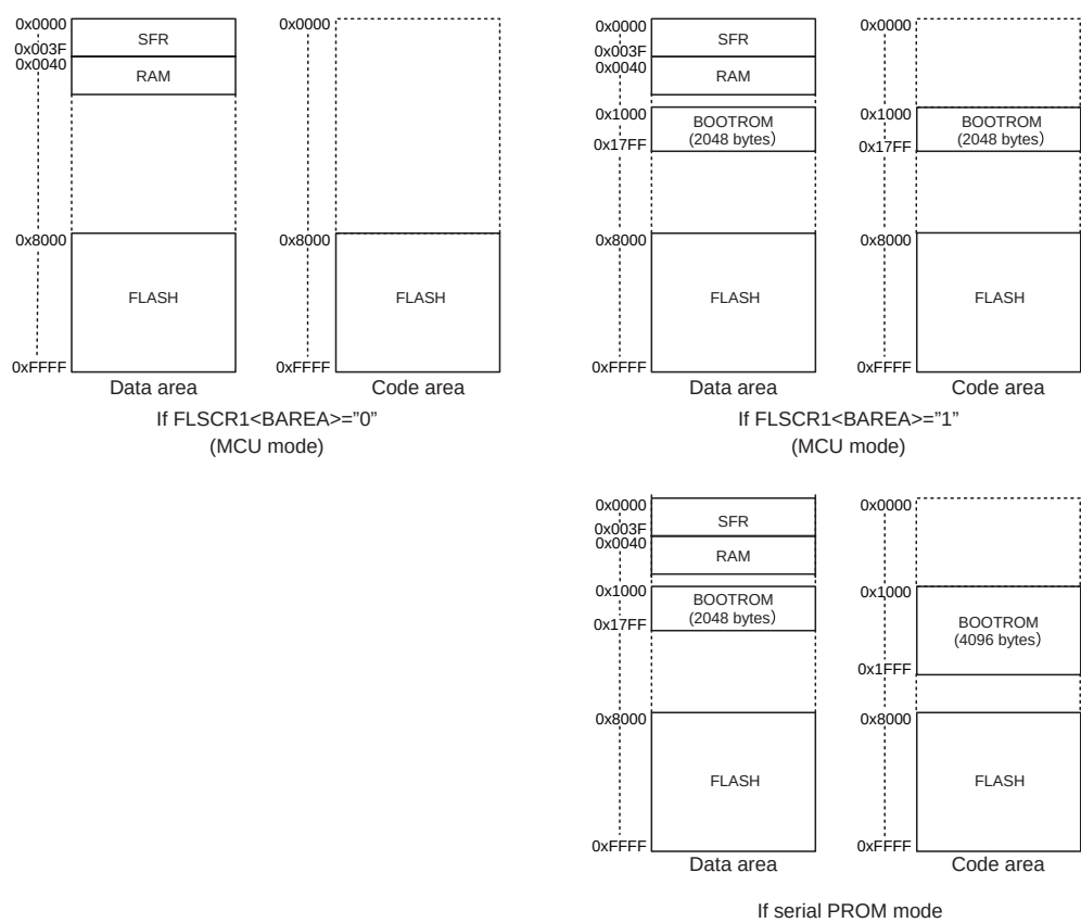
Figure 22-3 Memory Mapping
