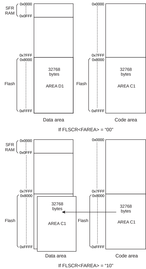
Figure 21-1 Area Switching Using the FLSCR1<FAREA> Setting
