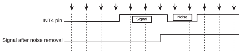
Figure 4-7 Noise Cancel Operation
