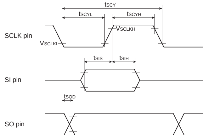
Figure 17-17 AC Characteristics
