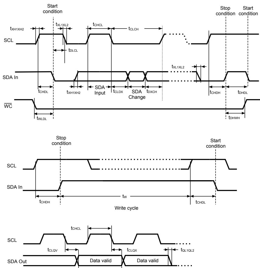
Figure 27. AC waveforms
