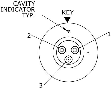
WIRE VIEW W17281-3PG-P-300
