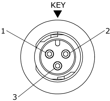
FACE VIEW W17281-3PG-P-300
