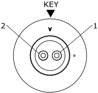
WIRE VIEW W17281-2PG-P-300
