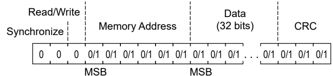
Figure 15: Write Sequence
