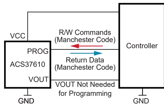
Figure 11: Programming Connections—Mode 2
