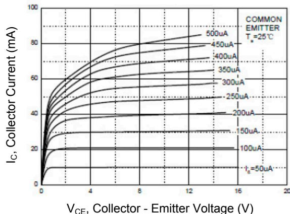
Figure 1. Static Characteristics
