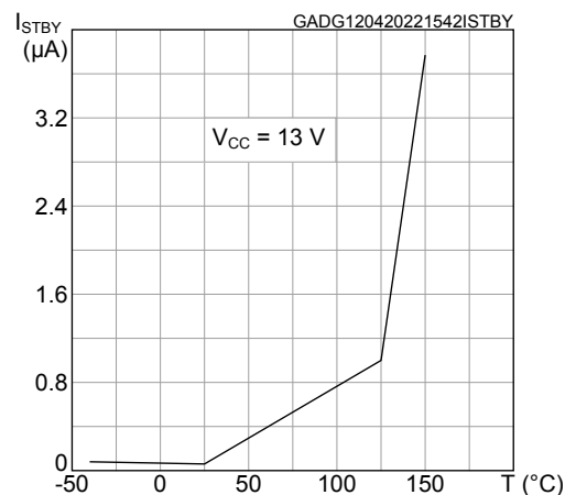
Figure 13. Standby current
