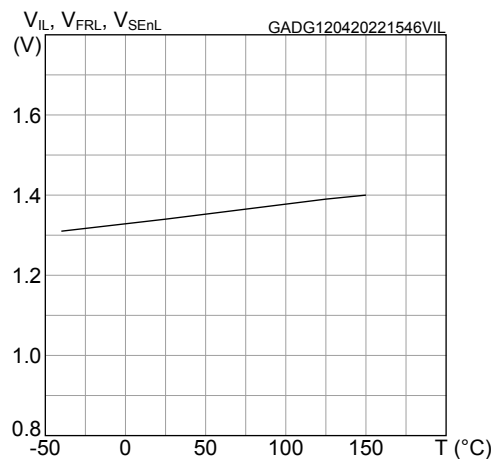
Figure 16. Logic input low level voltage
