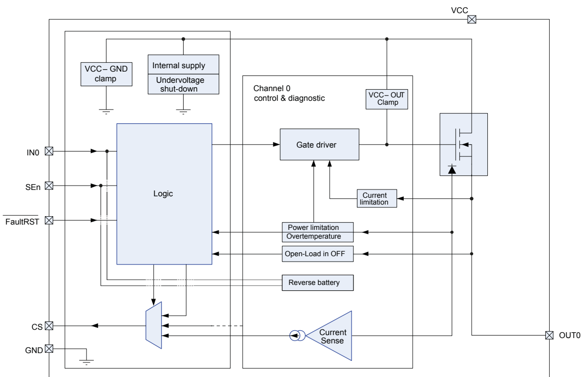
Figure 1. Block diagram
