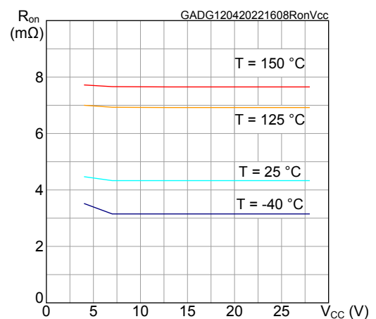
Figure 23. On-state resistance vs. V CC
