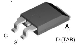
PLUS220SMD (IXFV__S)
