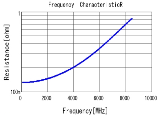
■ GCQ1555C1H3R7WB01 R DC0V, 25degC
