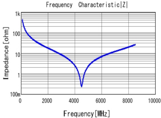
■ GCQ1555C1H3R7WB01 |Z| DC0V, 25degC
