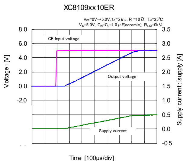
(16) Turn-on delay vs. Rise time ( C_L=1.0\mu\text{F} )
