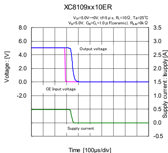
(17) Turn-off delay vs. Fall time ( C_L=1.0\mu\text{F} )
