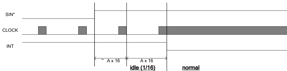
INT pin condition 2(idle → normal)
