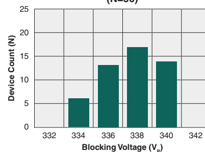
Typical Blocking Voltage Distribution (Form-A: I_F=0\text{mA} , Form-B: I_F=5\text{mA} ) (N=50)
