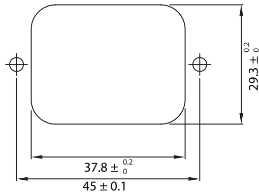
PANEL CUTOUT
