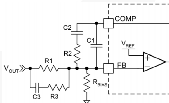
Figure 23. Compensation Network
