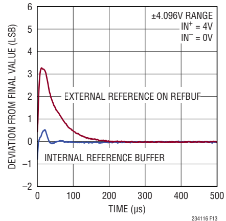
Figure 13. Burst Conversion Response of the LTC2341-16, f_{\text{SMPL}} = 666\text{ksps}
