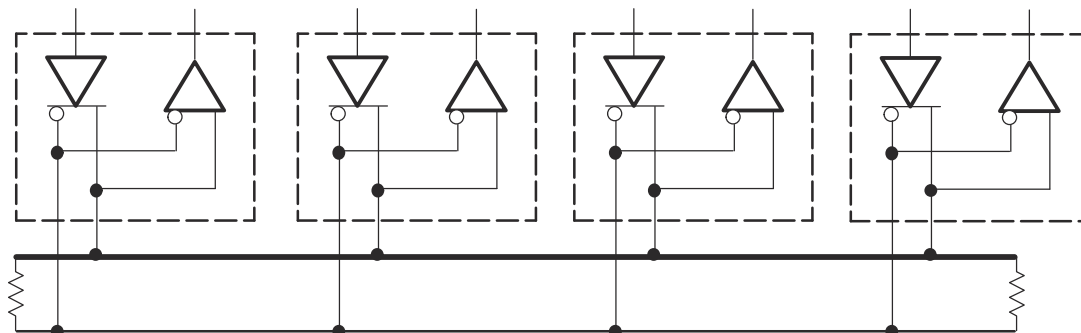
Figure 8-1. Multipoint Architecture
