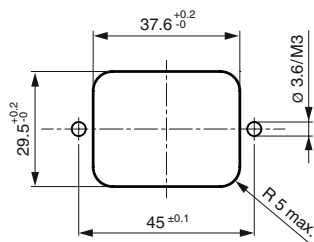
Panel cut-out for screw version
