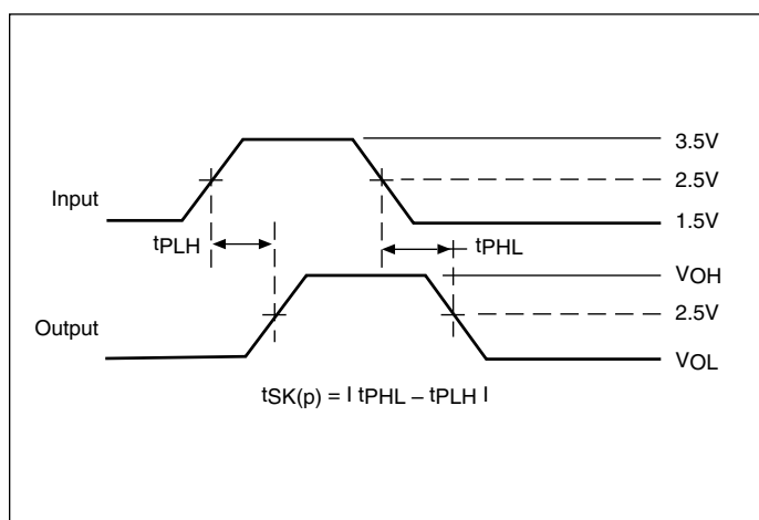
Pulse Skew - t_{SK(p)}
