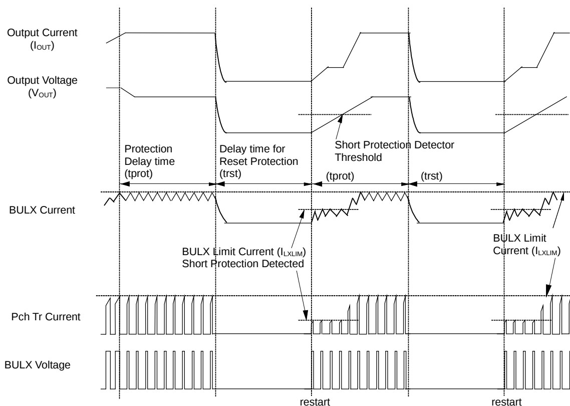
Timing Chart: RP602xxxxC/D/G/H Reset Protection Circuit
