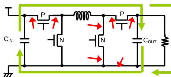
Figure 2. PMOSFET-ON (Step-up)
