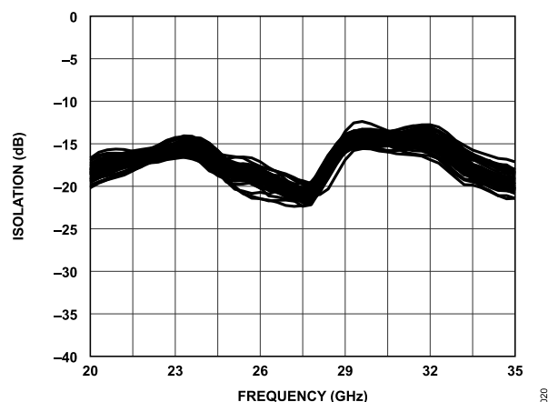
Figure 19. Distribution of Isolation Between Pin 2 and Pin 5 vs. Frequency for 50 Passive 3 × 3 Array Boards
