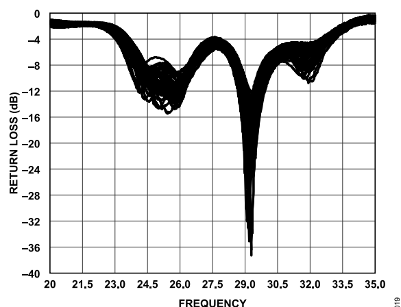
Figure 18. Distribution of Pin 5 Return Loss vs. Frequency for 50 Passive 3 × 3 Array Boards
