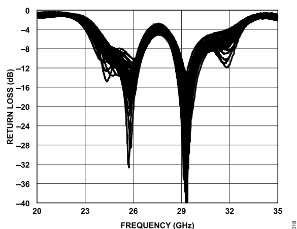
Figure 17. Distribution of Pin 2 Return Loss vs. Frequency for 50 Passive 3 × 3 Array Boards
