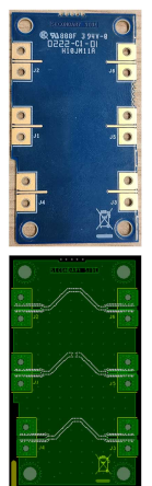
Figure 21. TRL Calibration Structure Used for Calibrating 3 \times 3 Antenna Array Evaluation Board (See Figure 20)
