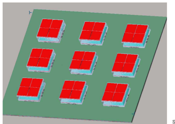
Figure 24. ANSYS HFSS Model of the 3 \times 3 Evaluation Board Shown in Figure 20
