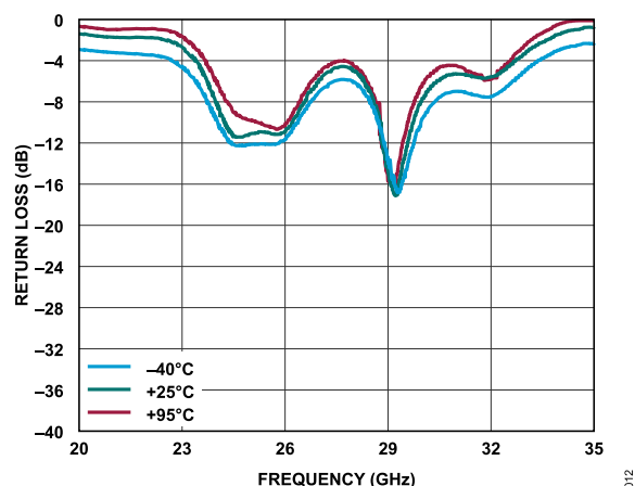
Figure 16. Pin 5 Return Loss vs. Frequency for a Passive 3 × 3 Array Configuration at Various Temperatures
