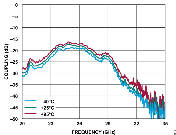
Figure 9. Pin 5 Coupling Crosspolarization vs. Frequency for a Passive 2 × 2 Array Configuration at Various Temperatures
