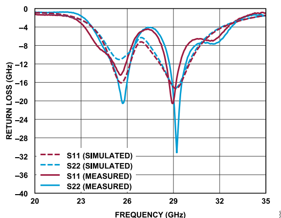
Figure 25. Simulated vs. Measured Pin 2 and Pin 5 Return Losses for the 3 \times 3 Passive Antenna Array Evaluation Board
