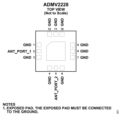
Figure 1. Pin Configuration
