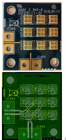
Figure 20. 3 \times 3 Passive Antenna Array of Pitch 5.25 mm in Both X-Axis and Y-Axis with a Central Radiating Antenna and Surrounding Antennas Acting as Parasitic Elements
