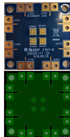
Figure 26. 2 \times 2 Passive Antenna Array of Pitch 5.25 mm in Both X-Axis and Y-Axis with Individually Measurable Antennas
